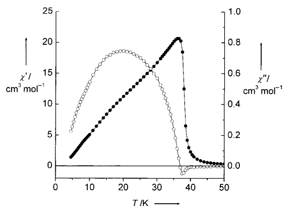
Figure 7. Real \chi' (●) and imaginary \chi'' (○) components of the ac susceptibility of 2 .
