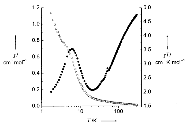
Figure 5. Plot of the susceptibility \chi (□) and \chi T (●) for 1 derived from field cooled measurements at 100 G.
