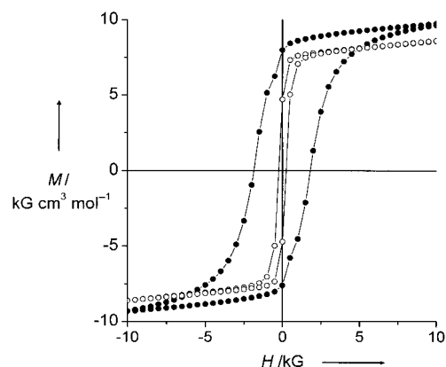
Figure 8. Hysteresis curve for 2 between \pm 10 \text{ kG} at 5 K (●) and 25 K (○).
